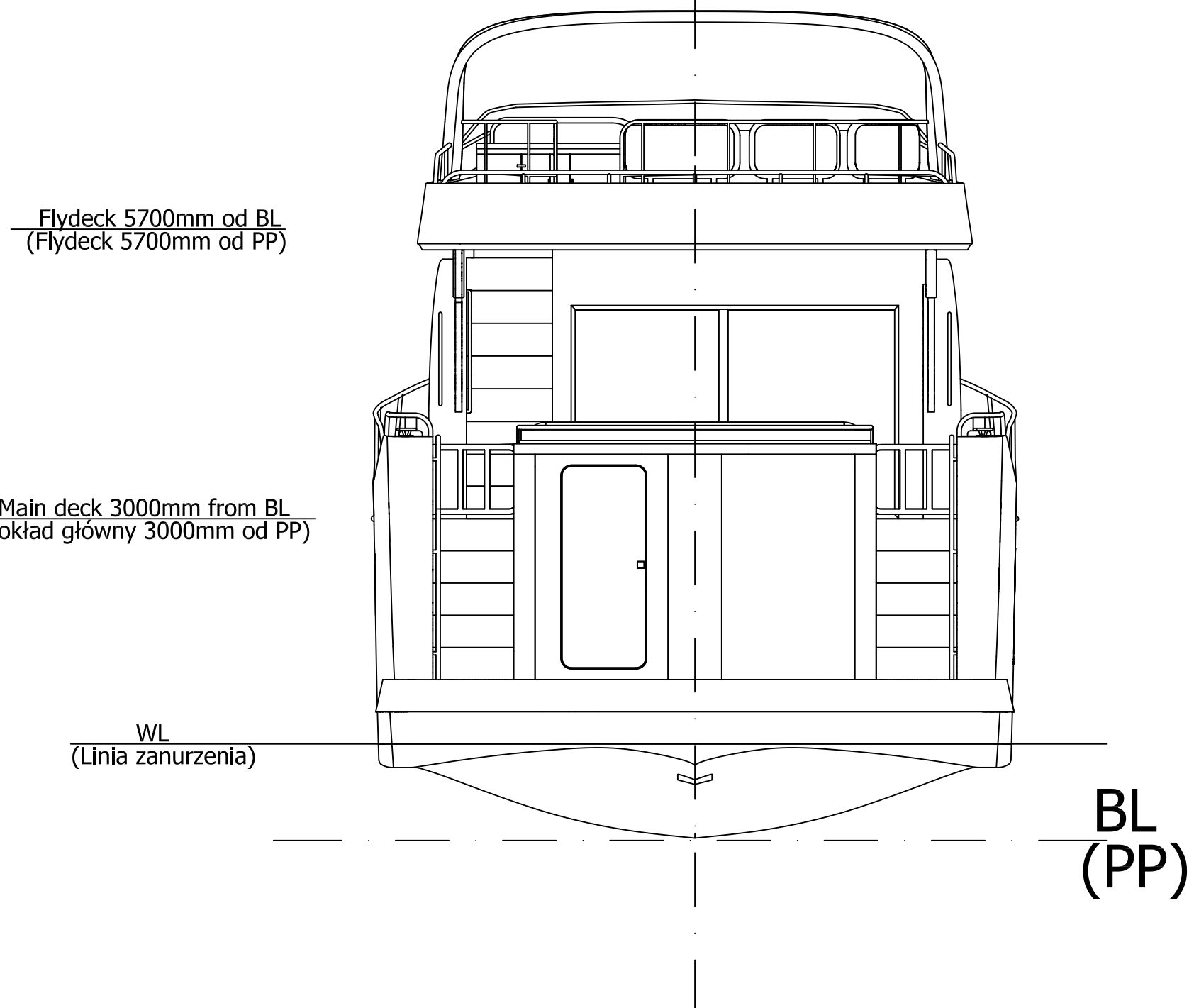
Stern view (Widok od rufy)
