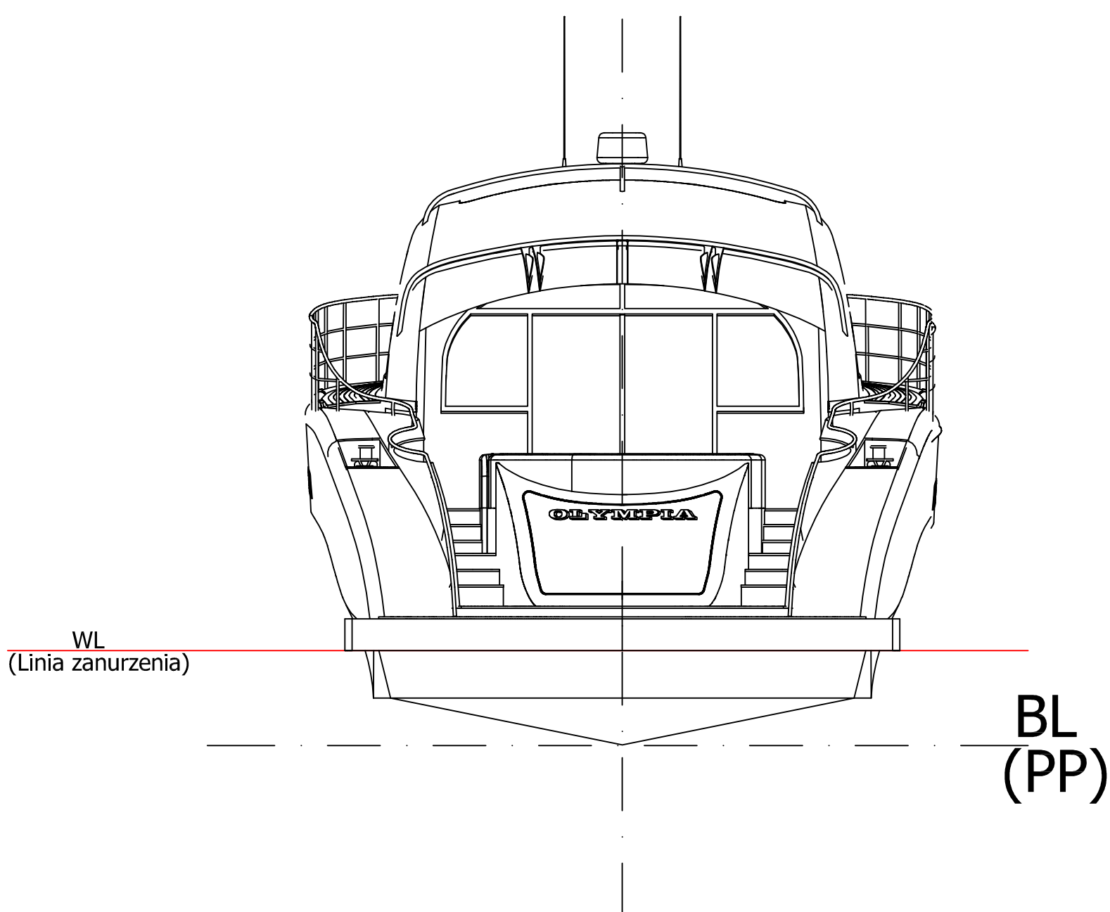
Stern view (Widok od rufy)
